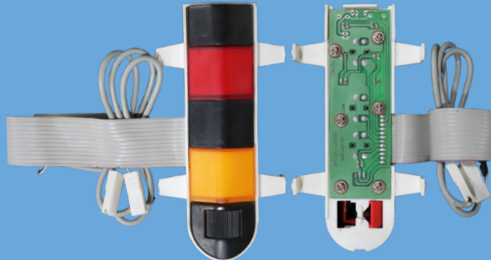
OPERATION SECTION'S WITH PCB
